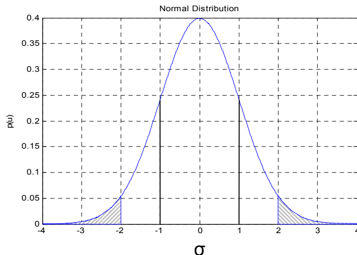
Fig. 15: Normal distribution
